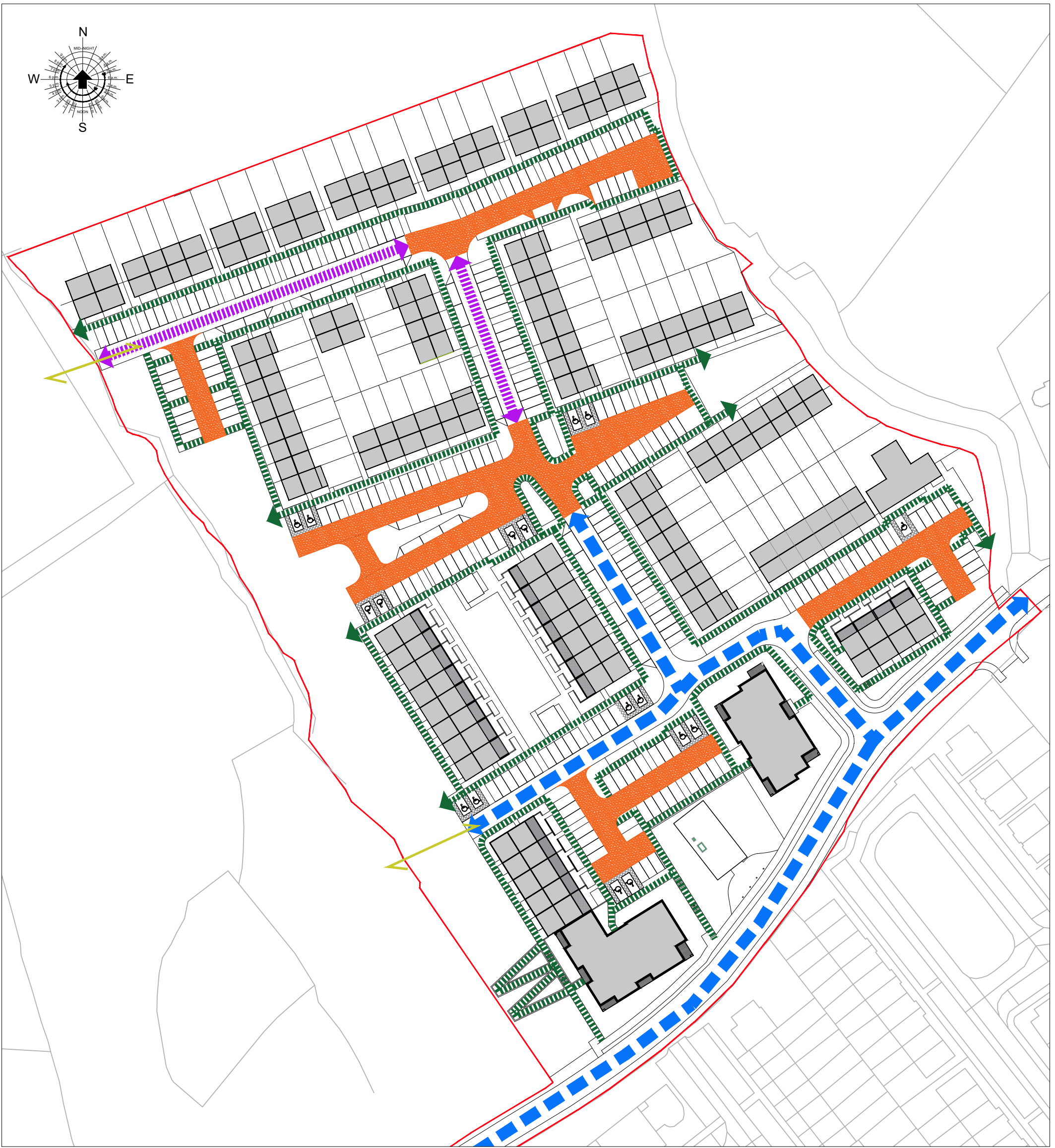
01 Site Connections & Street Hierarchy Diagram Scale: 1:1000
